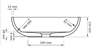
ON-TOP OVAL
