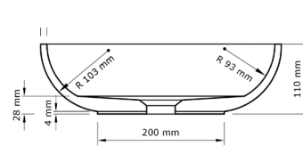
ON-TOP SQUARE
